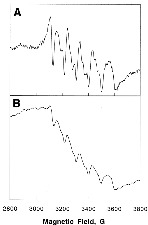
Fig. 3. X-band EPR spectra of 100 \mu\text{M} free manganese in solution (A) and iPGM (B). Experimental conditions: protein concentration in B, 2 mg/ml; temperature, 30 K; modulation amplitude, 5.2 Gauss; modulation frequency, 100 kHz; microwave frequency 9.42 GHz; microwave power 2.0 mW; receiver gain 2.5 \times 10^5 .
